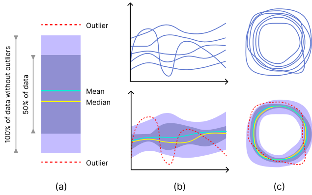
Fig. 1. Extension of the boxplot idiom (a) to the functional (b) and contour (c) data types.
