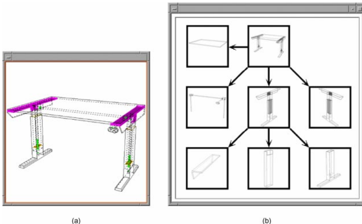
Fig. 2 Windows of a geometry camera for a table model (a), and a hierarchical graph camera for the table assembly (b)
