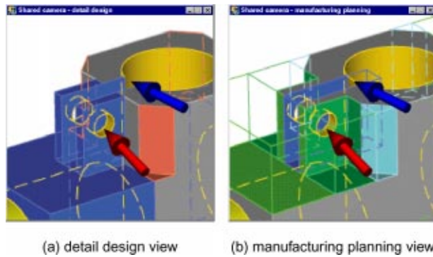
Fig. 6 Shared cameras of two team members with different views on the same part
