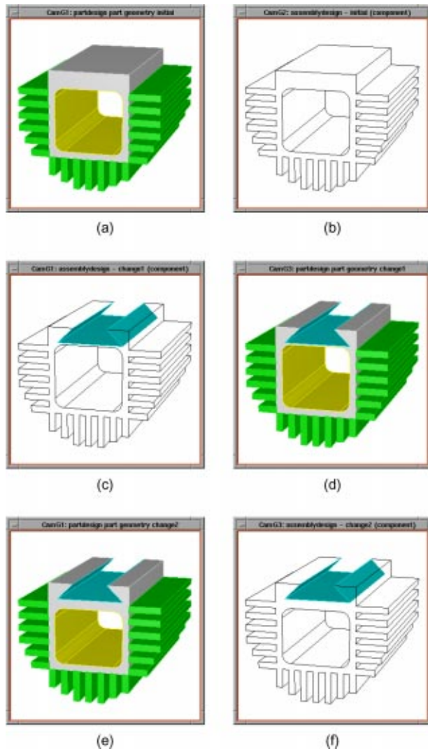
Fig. 3 If a detail design view on a part (a) and the assembly design view on the related component (b) become inconsistent because a form feature for a connection feature is added to the component (c), then the feature model of the part is updated accordingly (d). The resulting invalid feature model of the part is made valid again by reducing the height of the passage (e), thus increasing the distance between the passage and the new form feature, and the reference geometry of the component is updated accordingly (f).
