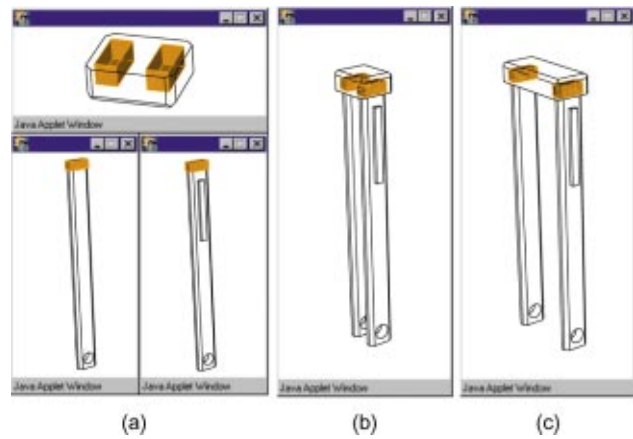
Fig. 8 Three components (a) are connected into the front fork assembly of a bicycle (b), of which the crown part is subsequently adjusted to make room for the front wheel (c)
