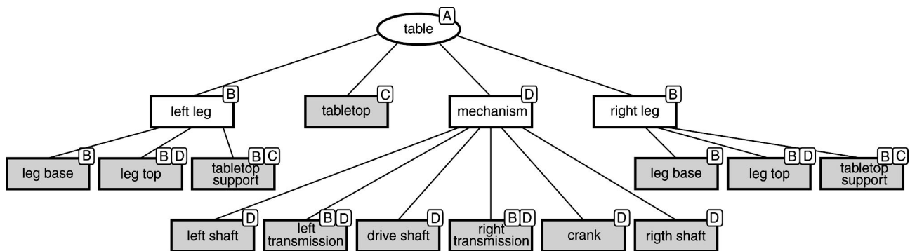
Fig. 10 Final task assignment for the fully specified product
